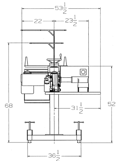
Thread Break Detectors Option
