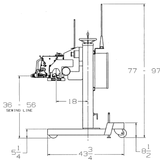
Needle Cooler Option
